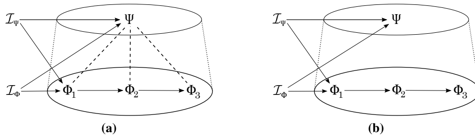
Figure 3: Two empirically indistinguishable mechanistic models.
